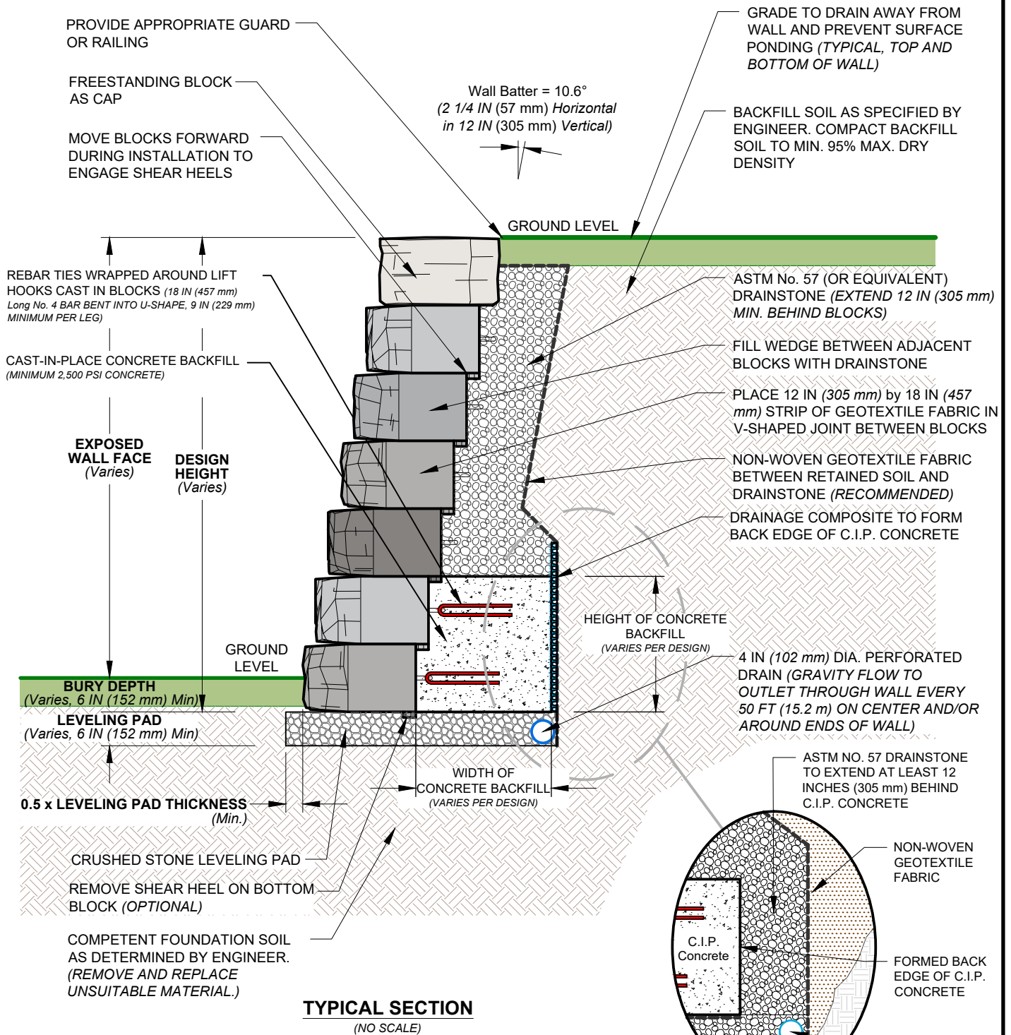
ALTERNATE DRAIN DETAIL BEHIND C.I.P. CONCRETE (NO SCALE)
