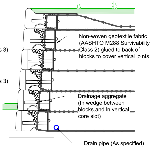
Typical Section - Option 2
