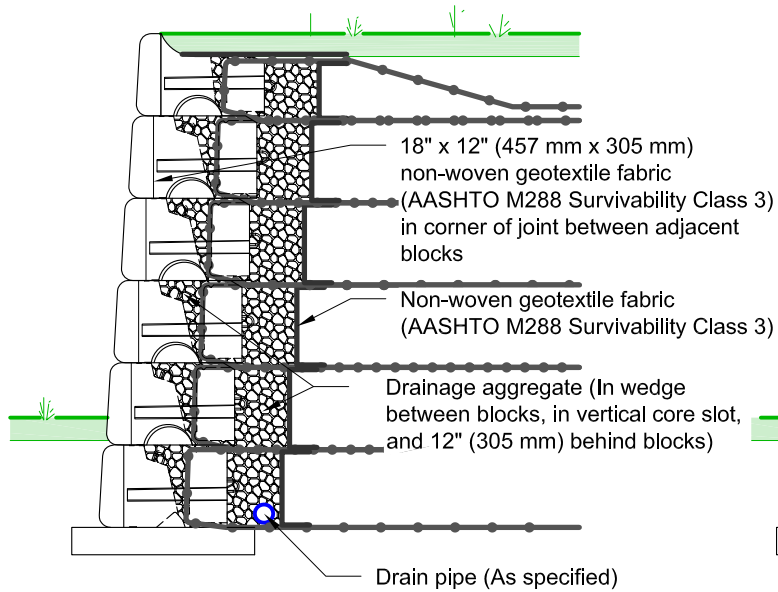
Typical Section - Option 1
